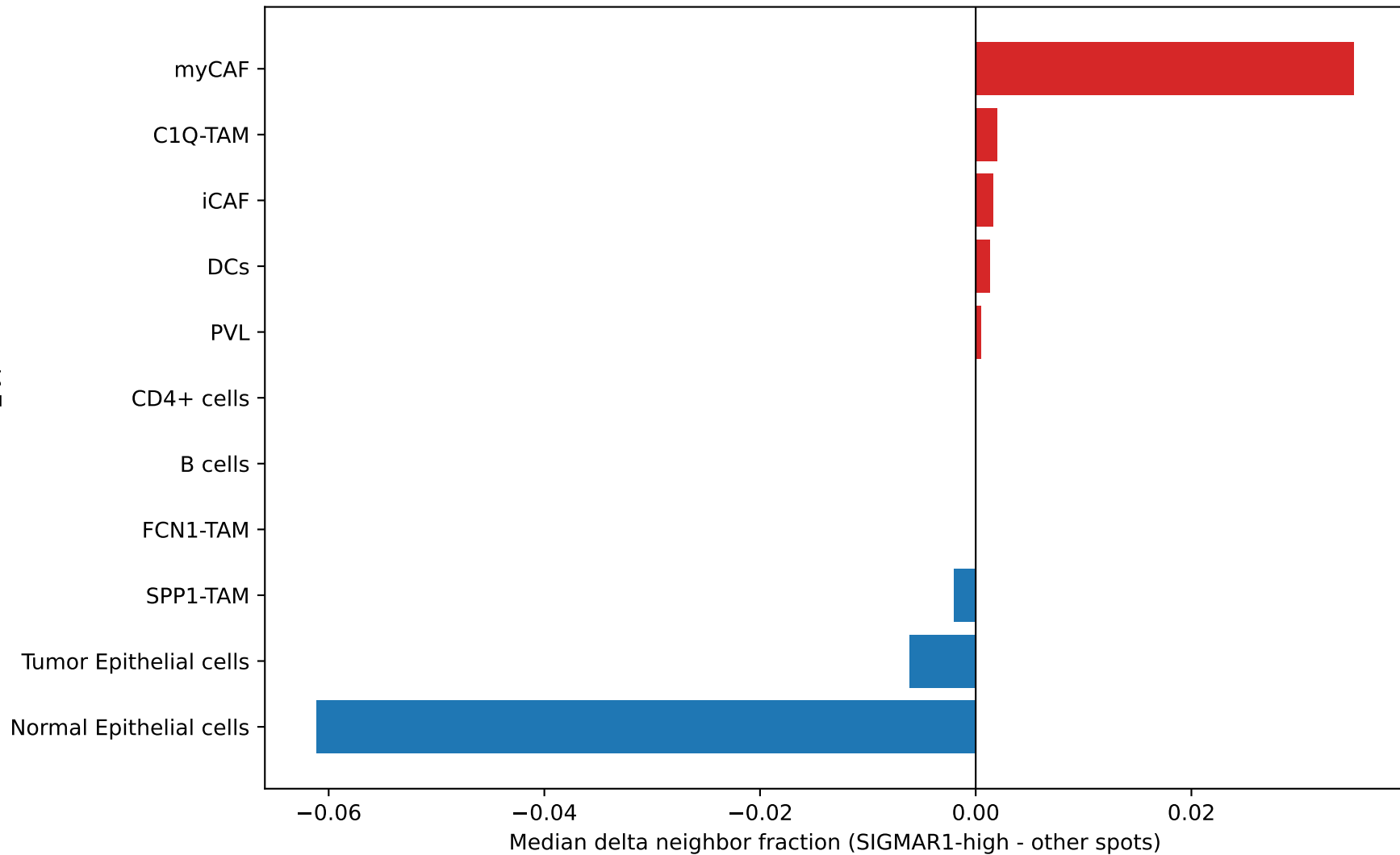
SIGMAR1: KNN neighborhood enrichment by cell type
