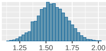
b_Intercept
