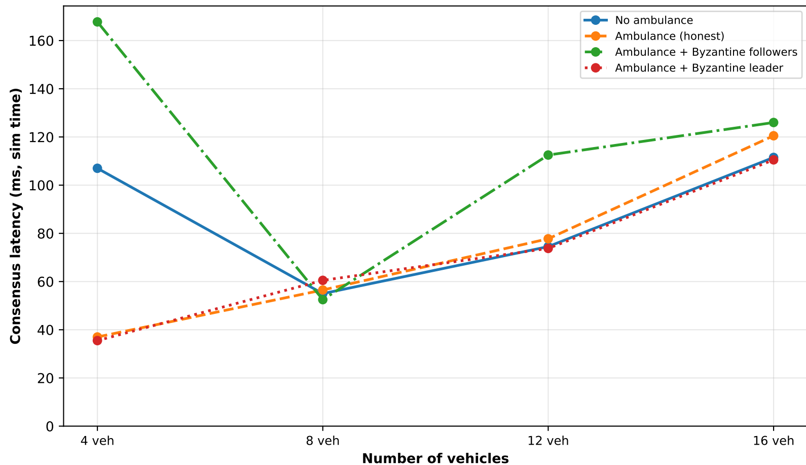
BFT-SMaRt intersection coordination (metrics from analyze_log JSON) BFT consensus latency by fleet size (overall.propose_all_consensus_latency_sim_s, sim time)
