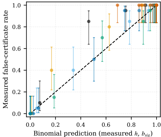
(b) Protocol-model validation
