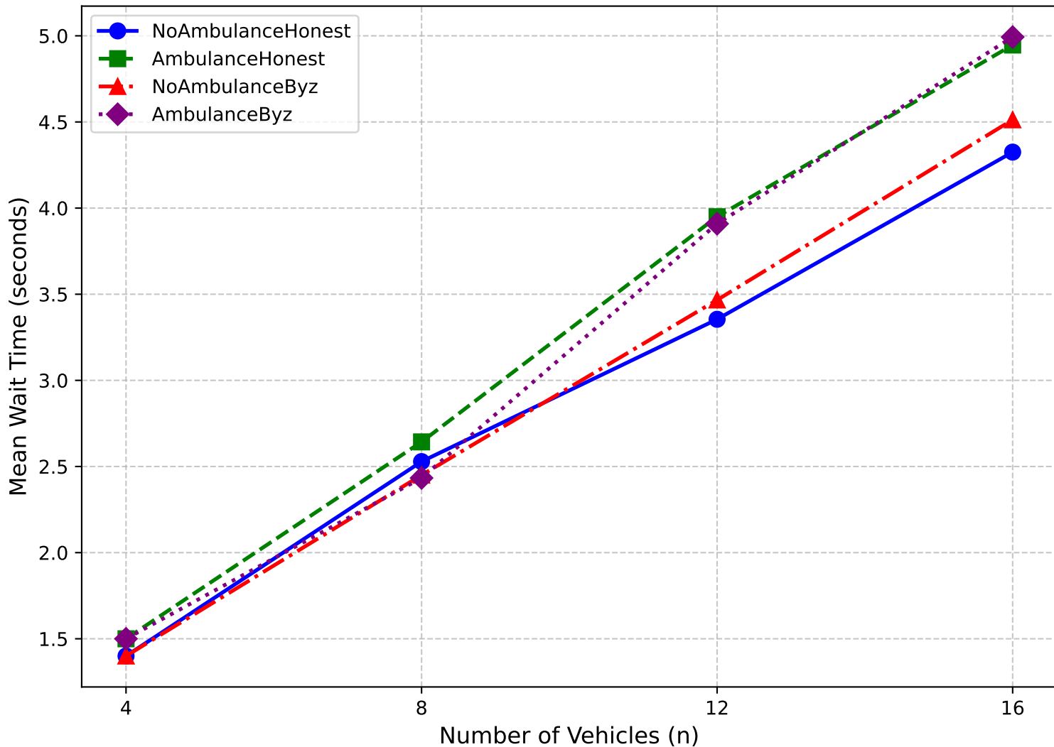
Mean Normal Vehicle Wait Time vs Total Vehicles
