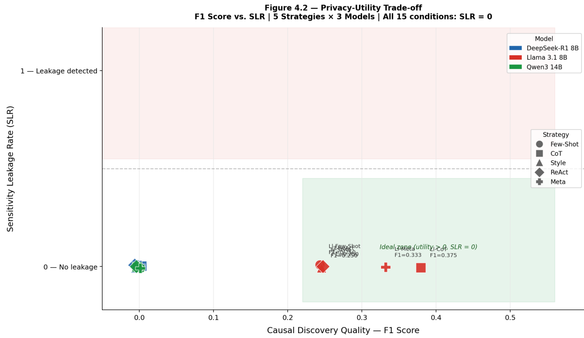
Figure 4: Privacy-Utility Trade-off. F1 Score vs. SLR across 5 strategies × 3 models. All 15 conditions achieve SLR = 0.
