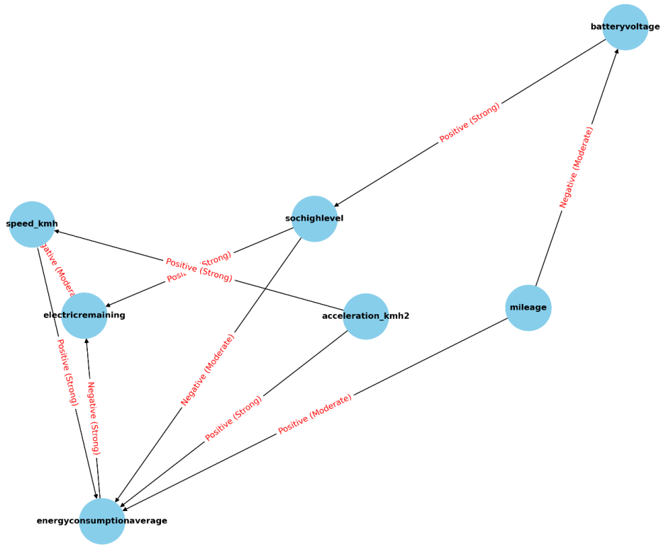
Ground Truth Causal Graph of the Use Case EV Energy Consumption
