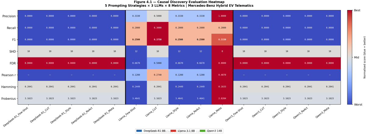
Figure 3: Causal Discovery Evaluation Heatmap. 5 Prompting Strategies × 3 LLMs × 8 Metrics on the Mercedes-Benz Hybrid EV Telematics dataset.
