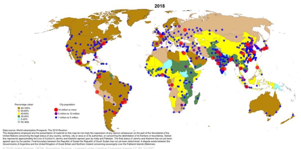
CityPop PercUrban-2018
