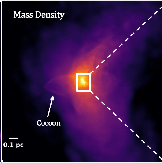
Face-on
