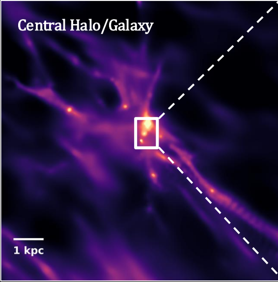
Mass Density
