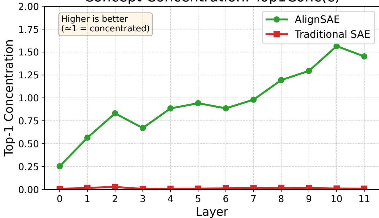
Concept Concentration: Top1Conc(c)
