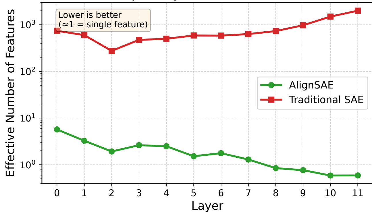
Concept Fragmentation: EffFeat(c)
