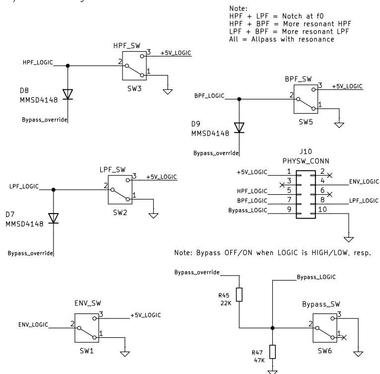
Physical SW configuration
