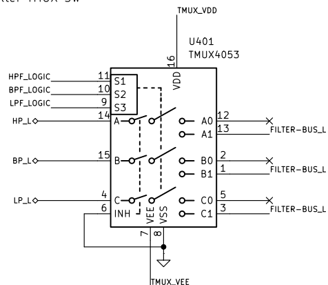
Filter TMUX SW
