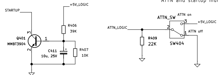
ATTN and startup mute
