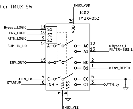
Other TMUX SW
