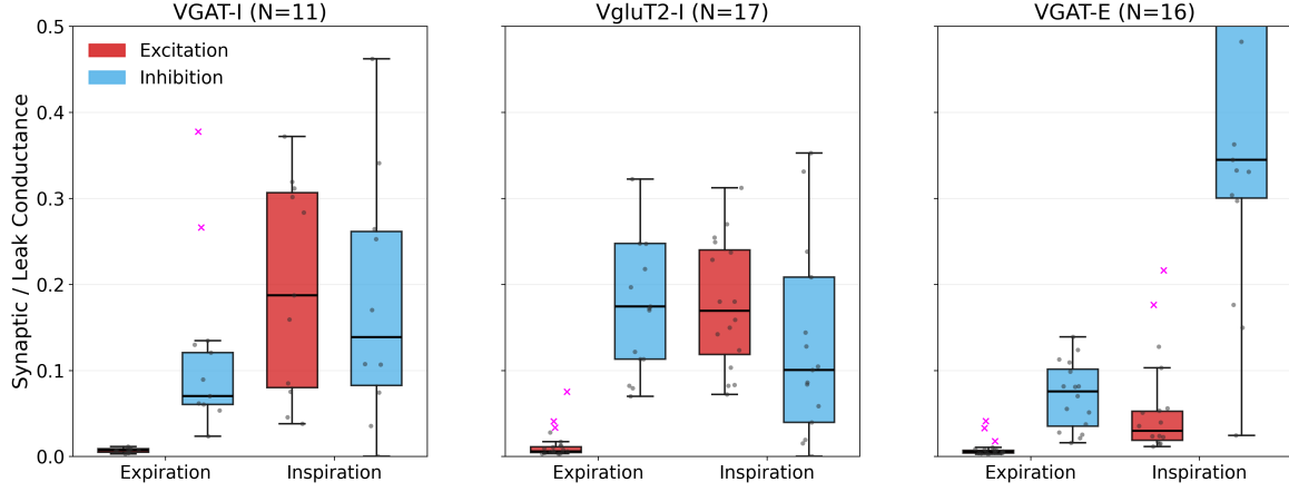
Figure 3: Population-level summary of excitatory and inhibitory conductances during expiration and inspiration for the three main groups (VGAT-I, VgluT2-I, VGAT-E). Box plots represent the median and interquartile range (IQR) of inliers, with whiskers extending to 1.5 times the IQR. Individual cells are overlaid as dots (inliers) and 'x' markers (outliers). Synaptic conductances are normalized to the leak conductance of each cell.
