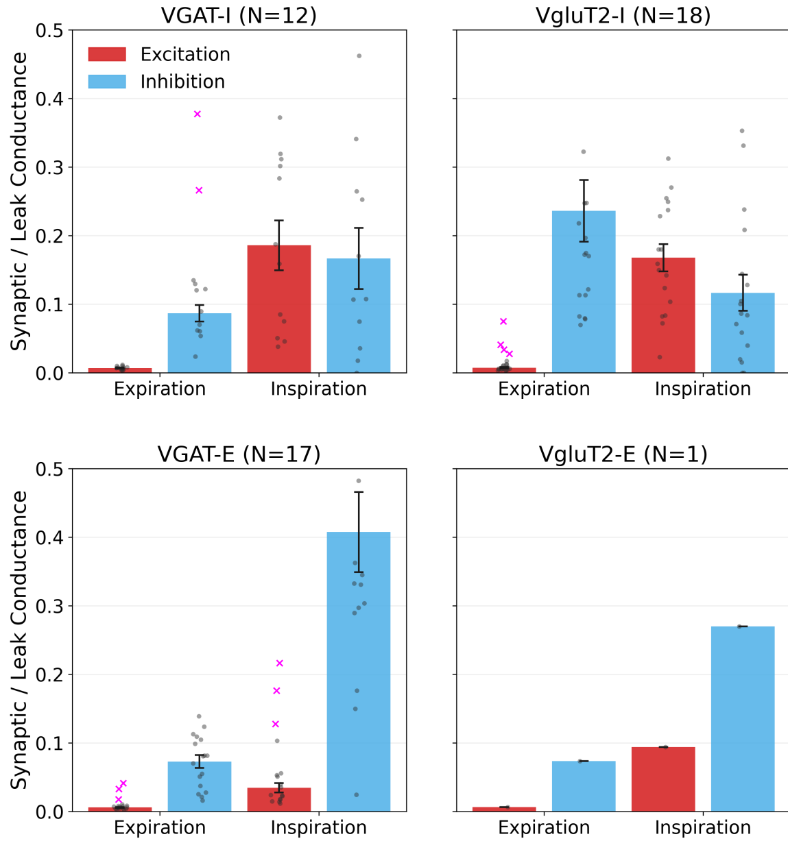
Figure 3: Population-level summary of excitatory and inhibitory conductances during expiration and inspiration for the four main groups (VGAT-I, VgluT2-I, VGAT-E, VgluT2-E). Bars represent mean \pm SEM of inliers. Outliers were detected and removed via the IQR method. Individual cells are overlaid as dots (inliers) and 'x' markers (outliers). Synaptic conductances are expressed in nS.
