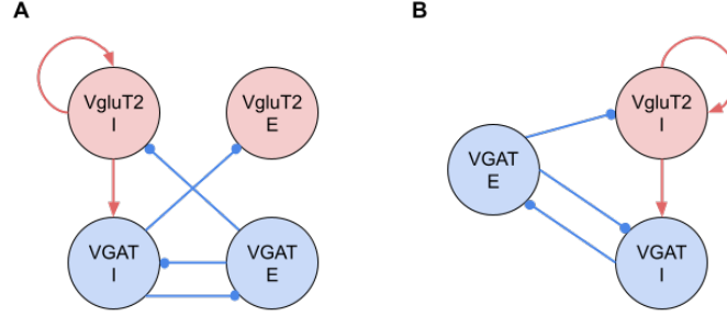
Figure 4: Proposed circuit diagram of preBötC connectivity inferred from synaptic conductance analysis. Red nodes/lines indicate (excitatory) components; Blue nodes/lines indicate (inhibitory) components. Arrows denote excitation; circles denote inhibition. (A) Complete connectivity graph comprising all four distinct populations defined by neurotransmitter type and firing phase. The VgluT2-I population provides recurrent and feed-forward excitatory drive (red arrows). Reciprocal inhibition (blue lines) enforces phase transitions: VGAT-I inhibits the Expiratory populations ( VgluT2-E , VGAT-E ) during inspiration, while VGAT-E inhibits the Inspiratory populations ( VgluT2-I , VGAT-I ) during expiration. Note that VgluT2-E receives phasic inhibition but does not provide significant synaptic output to other populations in this slice preparation. (B) The core rhythm-generating circuit. Excluding the non-driving VgluT2-E population highlights the essential “kernel” of the network: a self-exciting inspiratory source ( VgluT2-I ) coupled with a half-center oscillator formed by the mutually inhibitory VGAT-I and VGAT-E populations.
