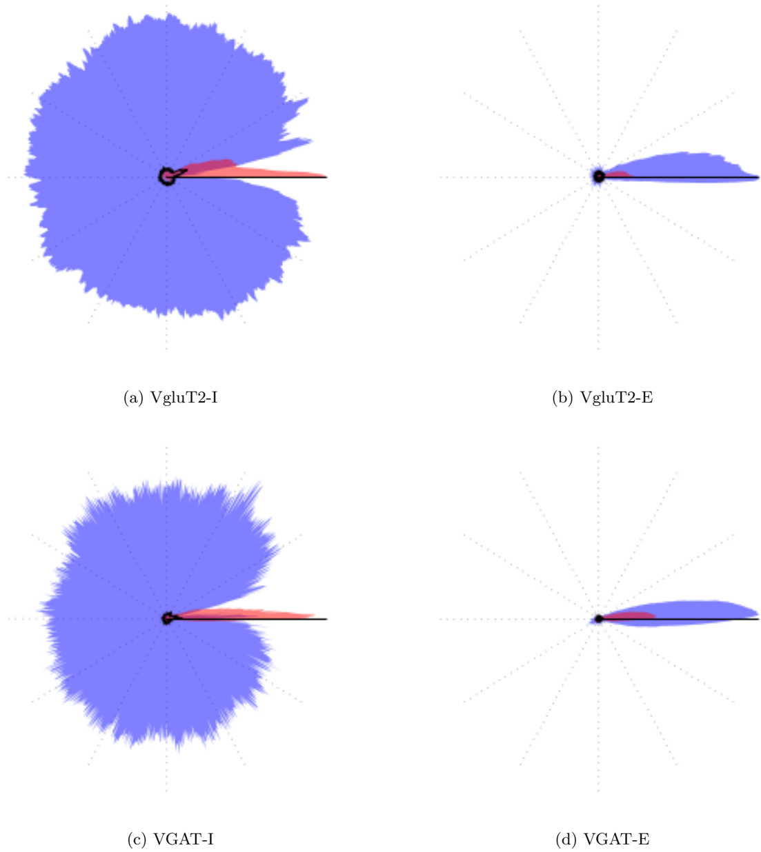
Figure 2: Representative cells for each neurotransmitter and firing phenotype. Panels exhibit inferred synaptic conductances for different cell types: (a) VgluT2 Inspiratory, (b) VgluT2 Expiratory, (c) VGAT Inspiratory, and (d) VGAT Expiratory. VgluT2 (vesicular glutamate transporter 2) indicates excitatory (glutamatergic) neurons, while VGAT (vesicular GABA transporter) indicates inhibitory (GABAergic/glycinergic) neurons.
