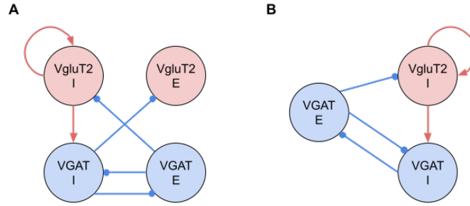
Figure 4: Proposed circuit diagram of preBötC connectivity inferred from synaptic conductance analysis. Red nodes/lines indicate (excitatory) components; Blue nodes/lines indicate (inhibitory) components. Arrows denote excitation; circles denote inhibition. (A) Complete connectivity graph comprising all four distinct populations defined by neurotransmitter type and firing phase. The VgluT2-I population provides recurrent and feed-forward excitatory drive (red arrows). Reciprocal inhibition (blue lines) enforces phase transitions: VGAT-I inhibits the Expiratory populations (VgluT2-E, VGAT-E) during inspiration, while VGAT-E inhibits the Inspiratory populations (VgluT2-I, VGAT-I) during expiration. Note that VgluT2-E receives phasic inhibition but does not provide significant synaptic output to other populations in this slice preparation. (B) The core rhythm-generating circuit. Excluding the non-driving VgluT2-E population highlights the essential “kernel” of the network: a self-exciting inspiratory source (VgluT2-I) coupled with a half-center oscillator formed by the mutually inhibitory VGAT-I and VGAT-E populations.
