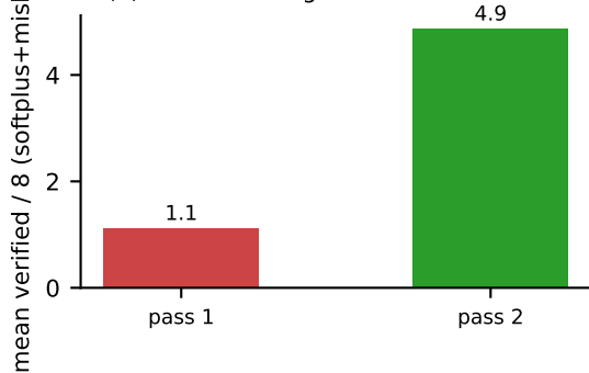
(b) the overflow-guard idiom is learned
