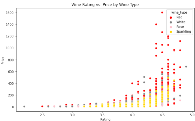
Figure 2: Rating vs. Price by Wine Type
