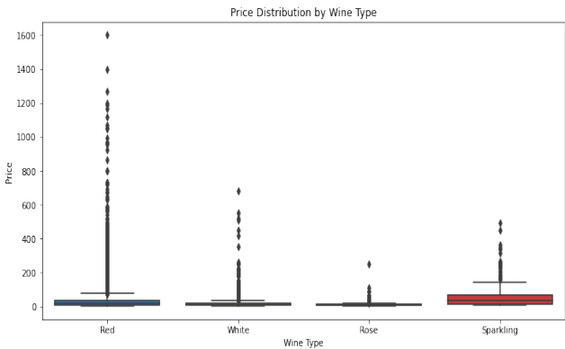
Figure 3: Price Distribution by Wine Type
