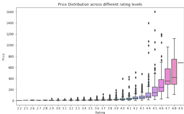
Figure 1: Price Distribution by Rating Level
