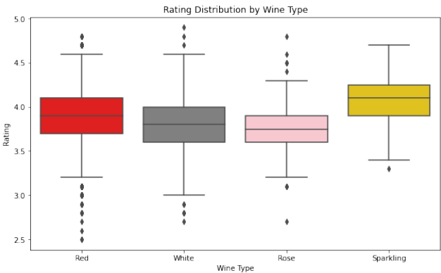
Figure 4: Rating Distribution by Wine Type
