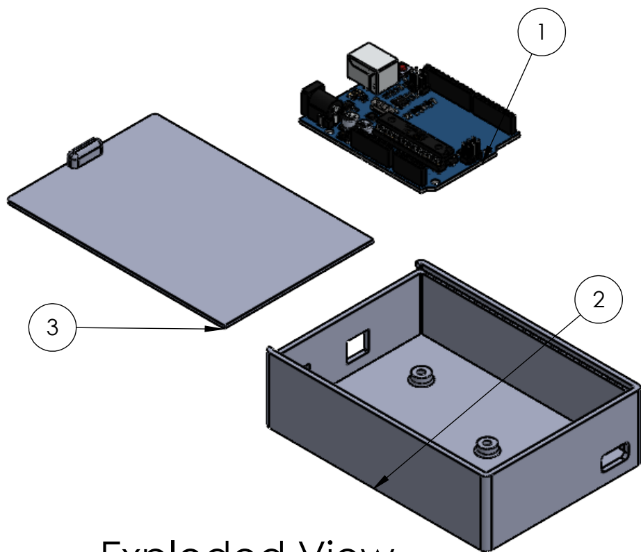
Exploded View
