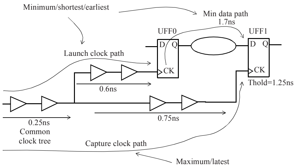
Figure 10-2 Derating hold timing check for OCV.
