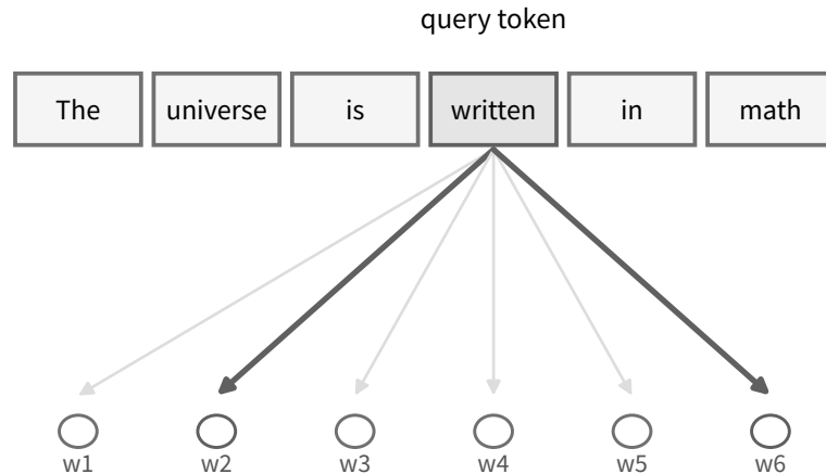
(b) AI：Self-Attention
