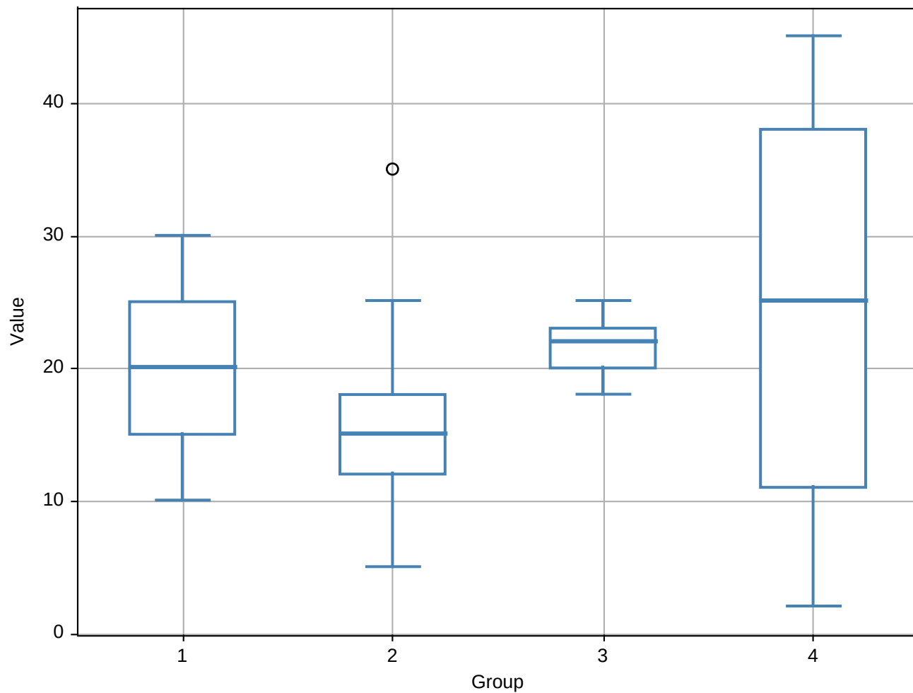
Box and Whisker Plot ? 4 Groups
