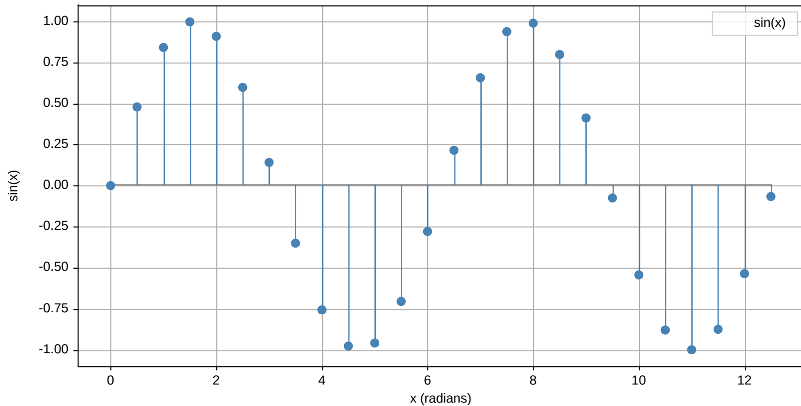
Stem Plot ? \sin(x)
