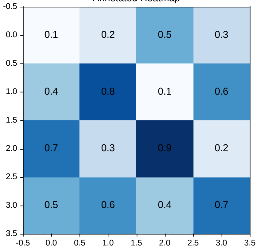
Annotated Heatmap
