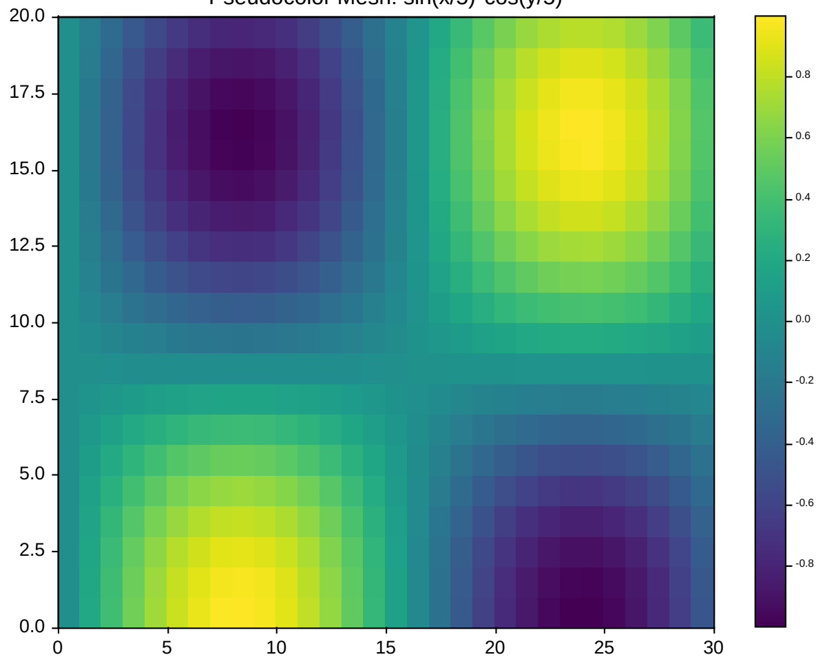
Pseudocolor Mesh: \sin(x/5)*\cos(y/5)
