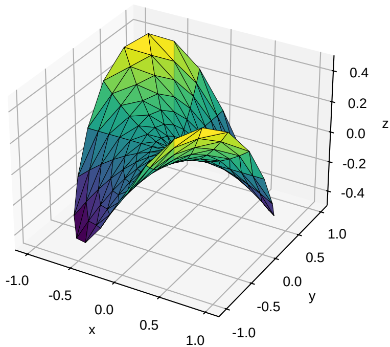
triangulated surface
