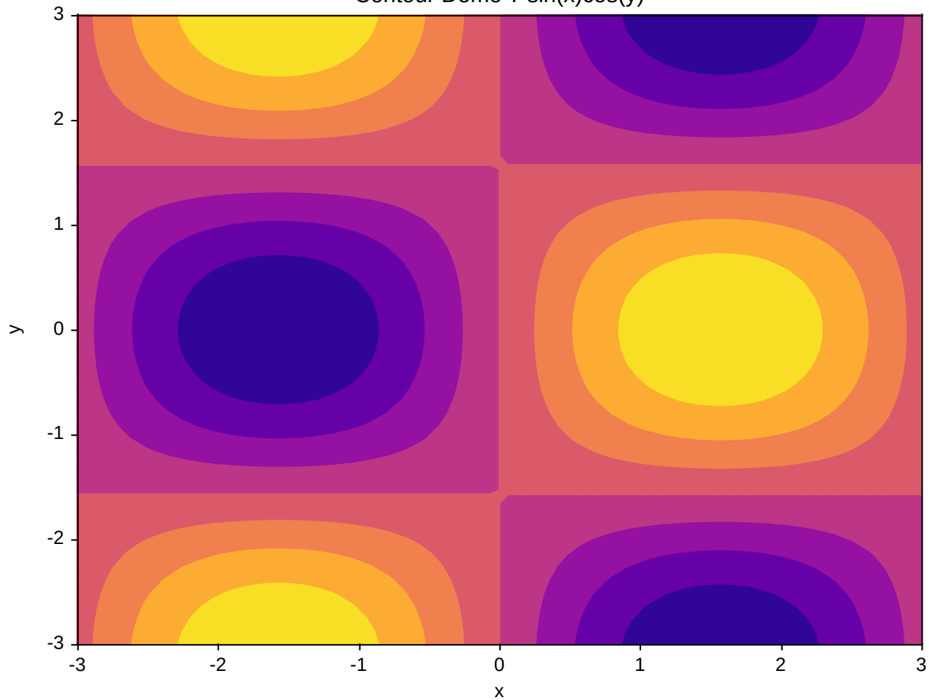
Contour Demo ? \sin(x)\cos(y)
