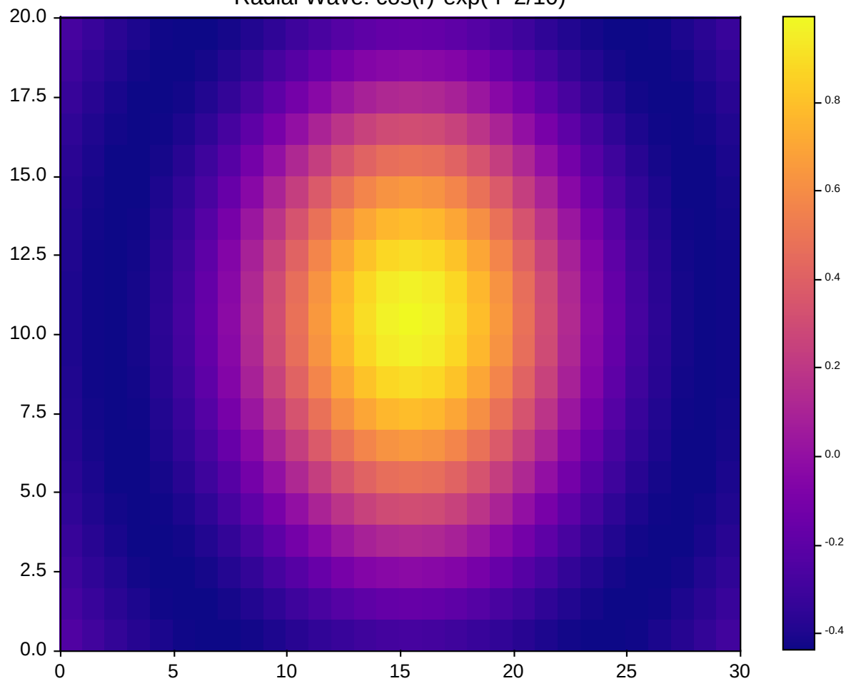
Radial Wave: \cos(r) \cdot \exp(-r^2/10)
