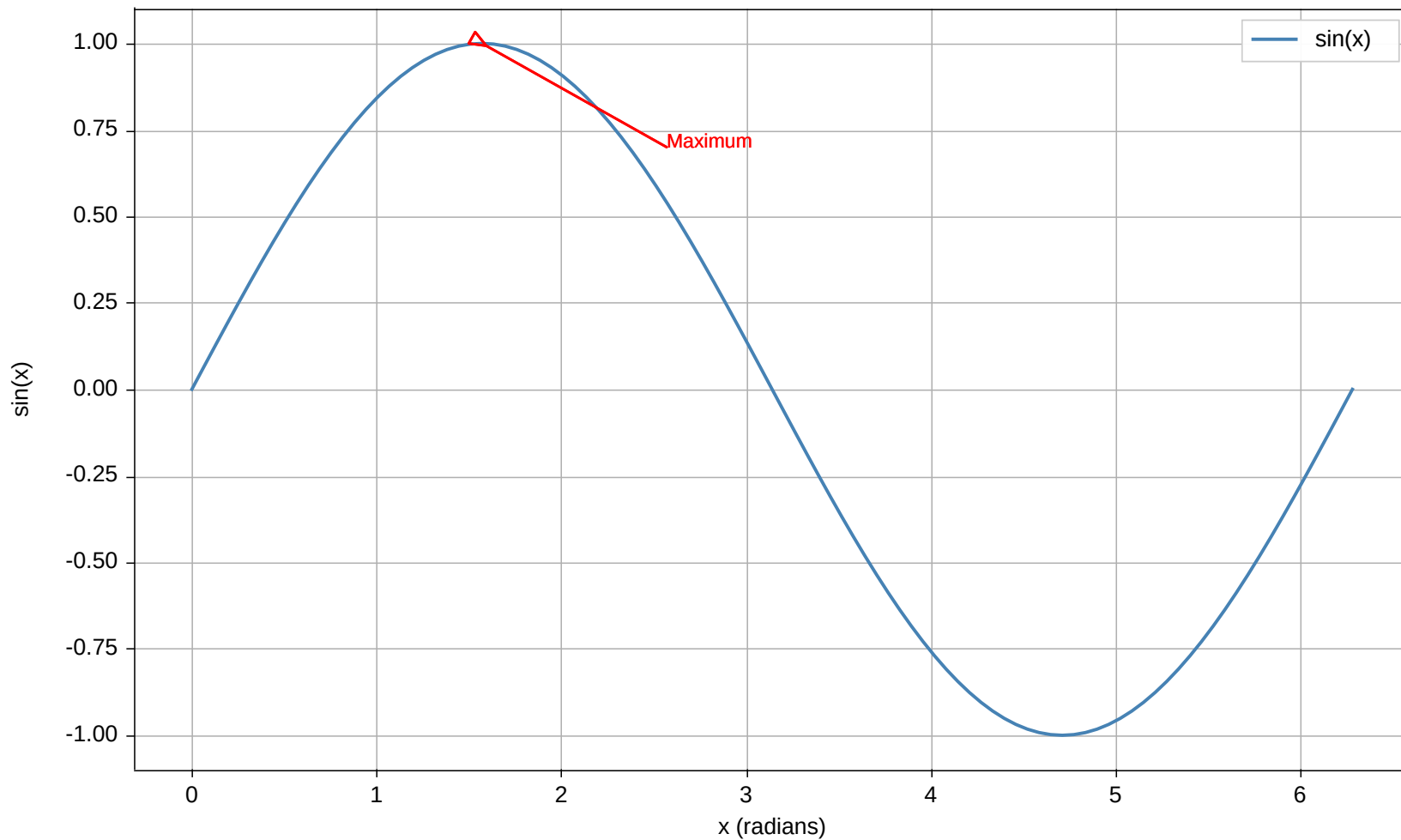
Annotated Plot of \sin(x) with Peak
