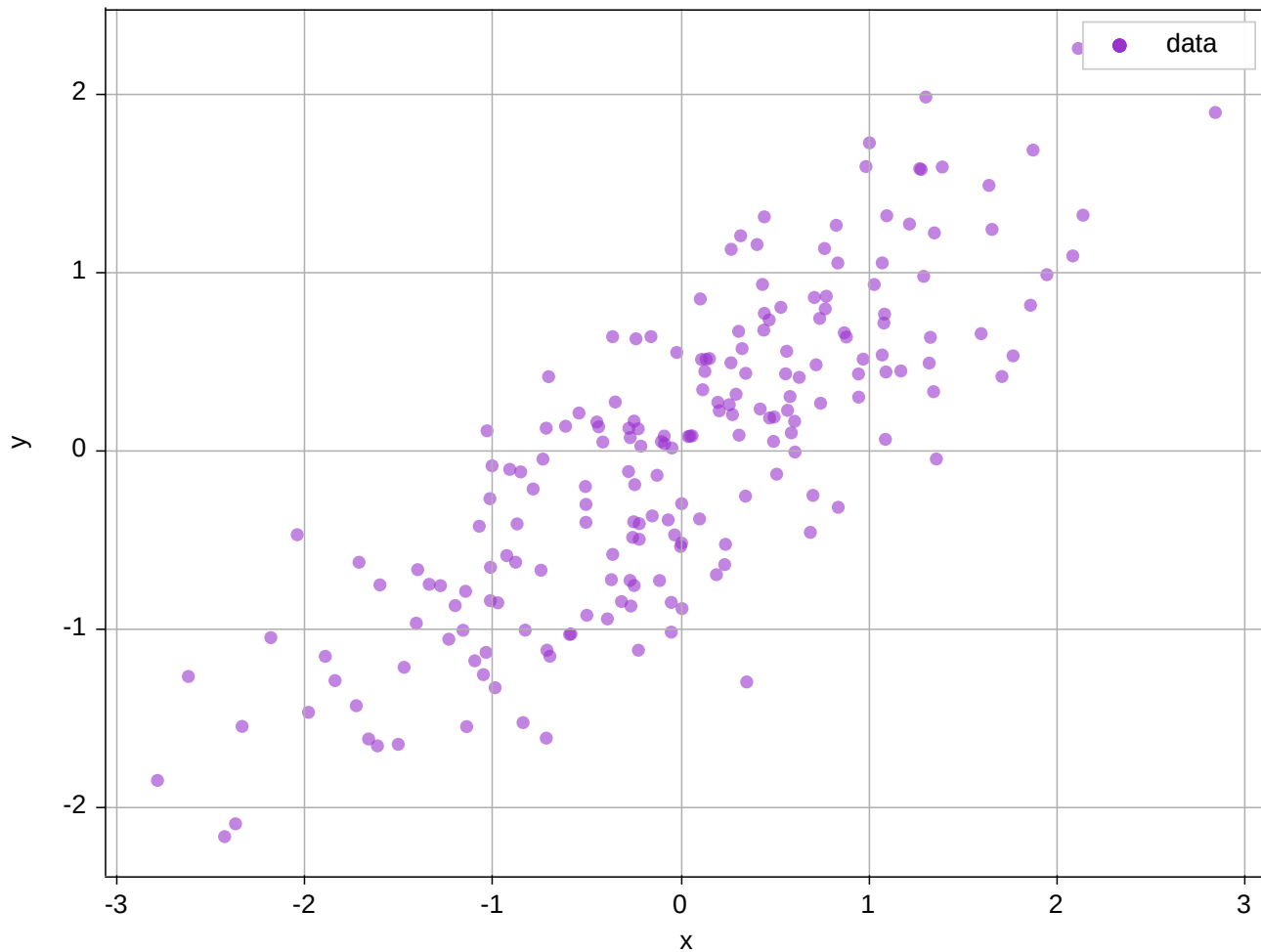
Scatter Plot
