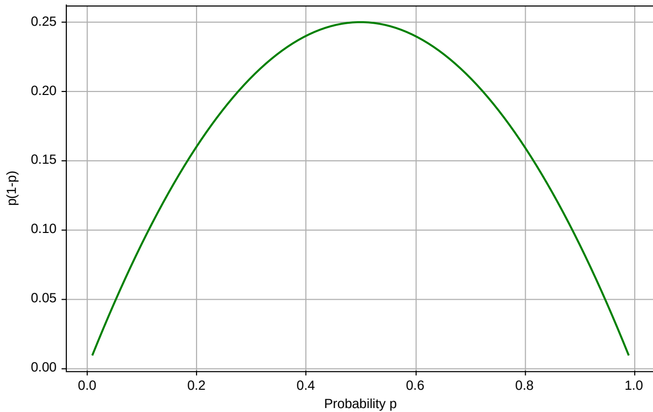
Probability Product p(1-p)
