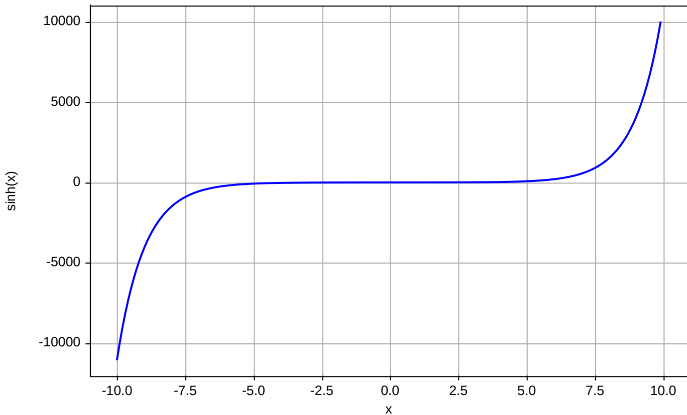
\sinh(x) ? Hyperbolic Sine
