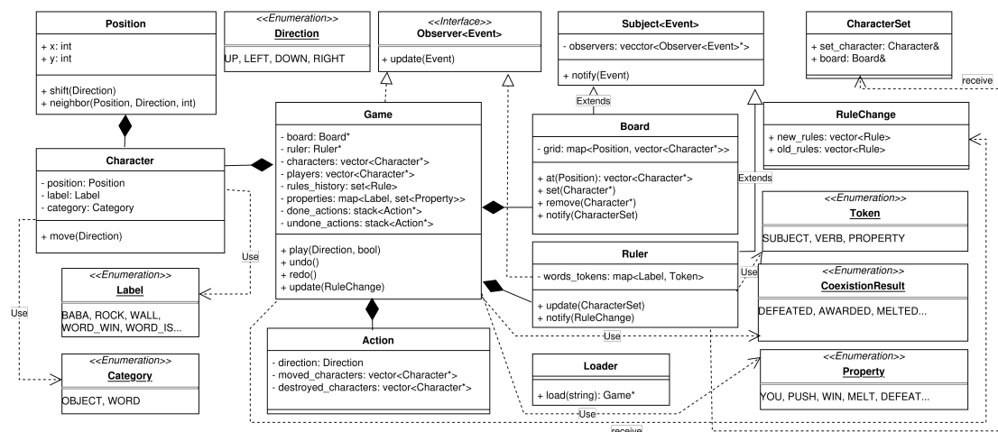
Figure 1: Diagramme UML
