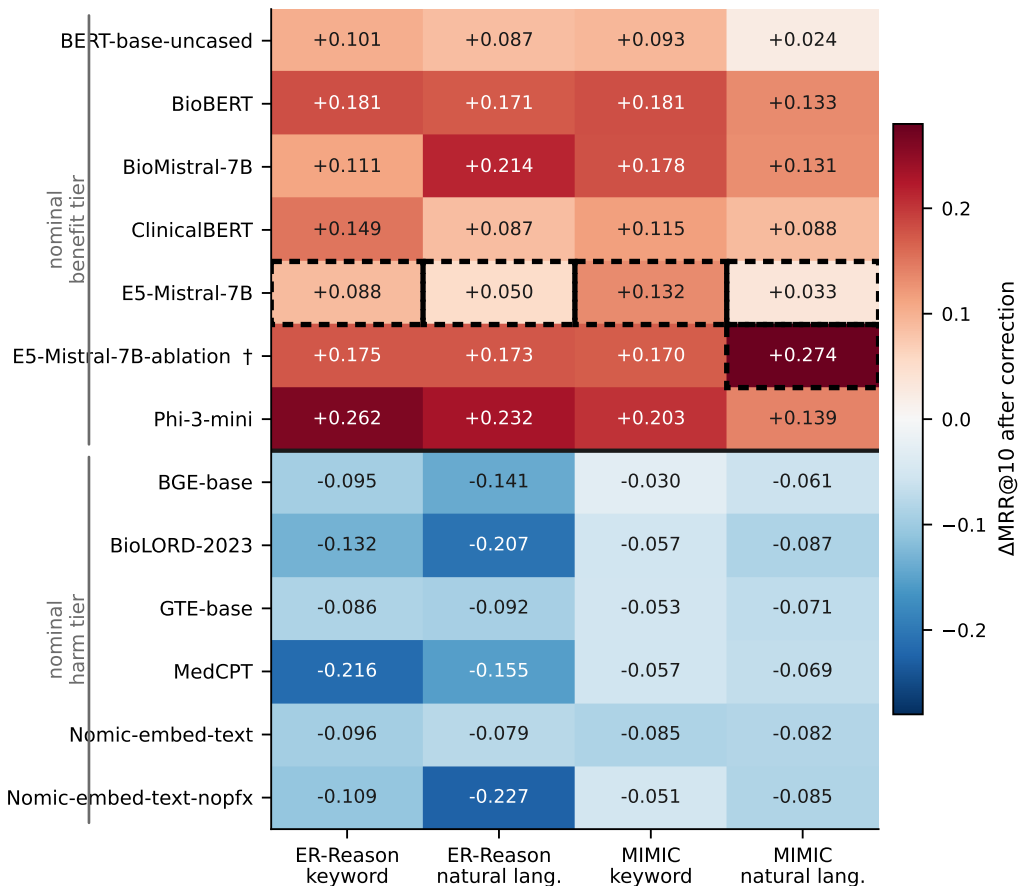
Measured response ( \Delta\text{MRR}@10 ) by deployment condition
