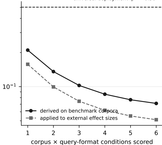
A. Cross-condition evidence breadth universal deployment p^* = 0.50
