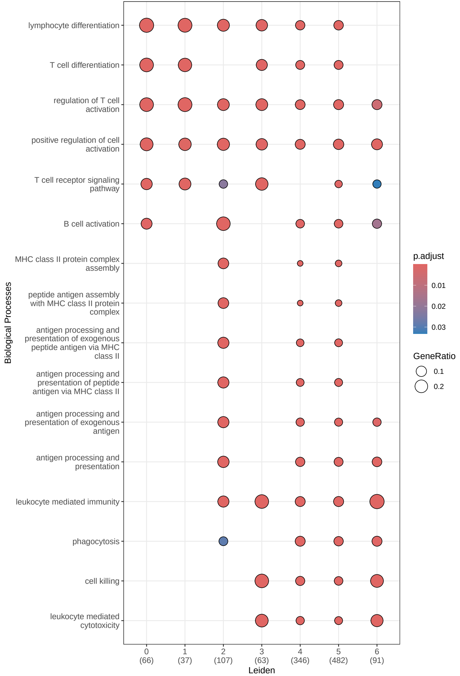
GO Enrichment across Clusters
