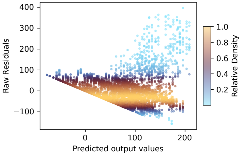
Model \Phi
