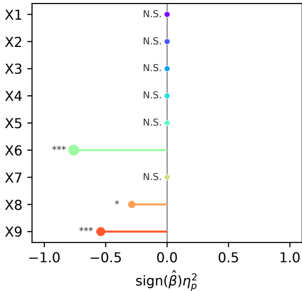
Model \Phi + C+LOO design (N=3)
