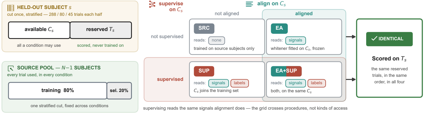
Fig. 1. Left: the two divisions of the data, each made once and identical in every condition. Right: the four conditions as a 2 \times 2 over the two procedures, with what each reads from the held-out subject’s available half C_s . Supervised training necessarily reads those trials’ signals as well as their labels, so the grid crosses two procedures , not two independent kinds of access. Everything else is held fixed: the source training set, the selection set, the samples drawn per epoch and the expected target share of a batch, and all four are scored on the same reserved trials in the same order.
