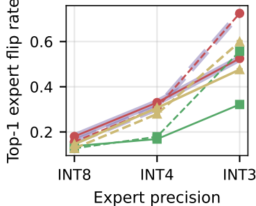
Top-1 expert changes
