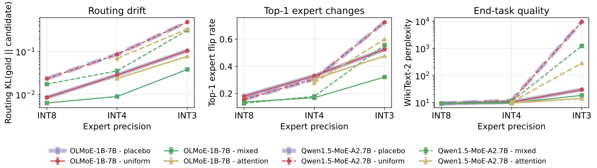
Protecting the router alone, across two MoE architectures
