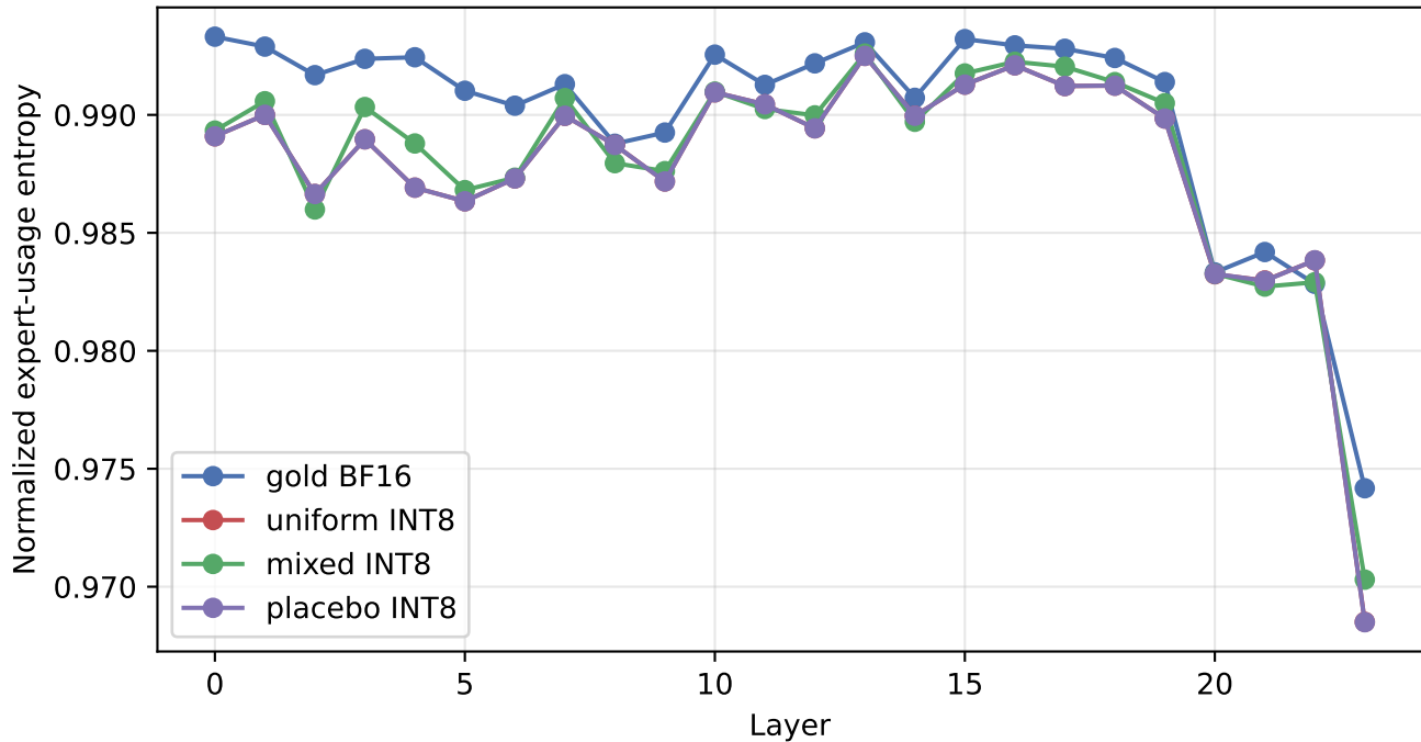
qwen: per-layer usage entropy at INT8
