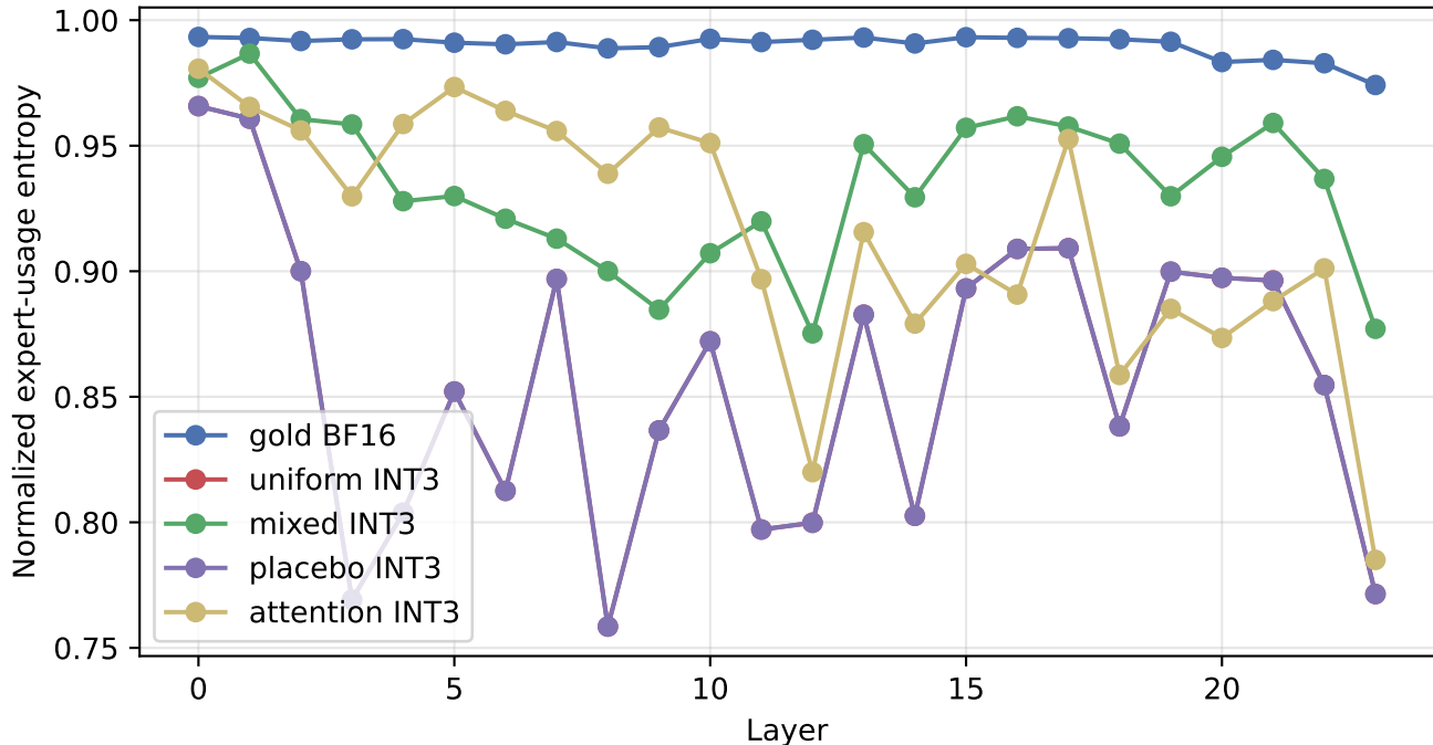
qwen: per-layer usage entropy at INT3
