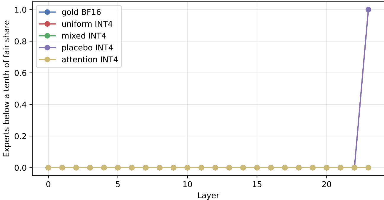
qwen: starved experts by layer at INT4
