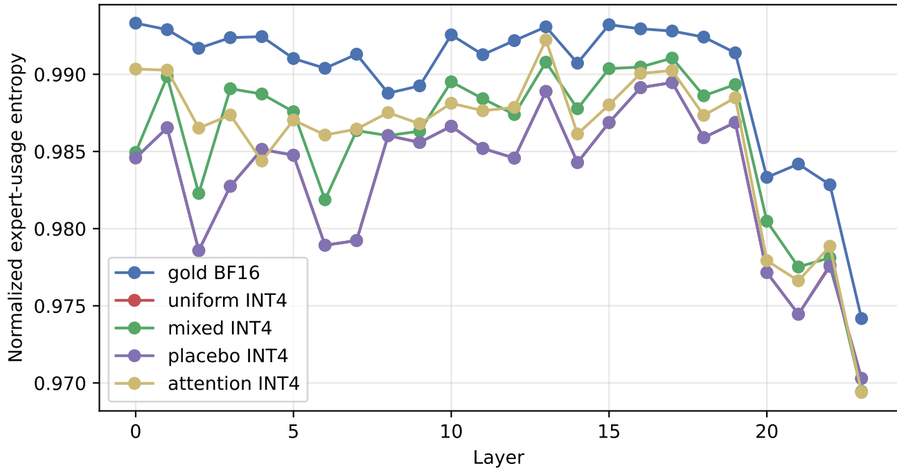
qwen: per-layer usage entropy at INT4
