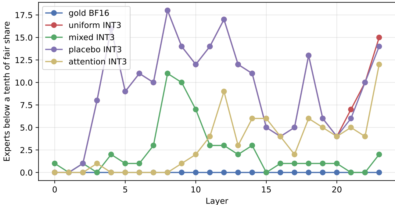
qwen: starved experts by layer at INT3
