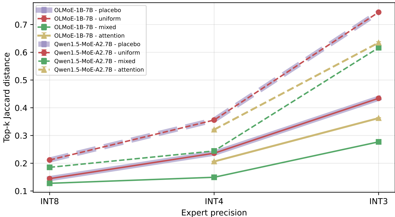
Top-k Jaccard distance
