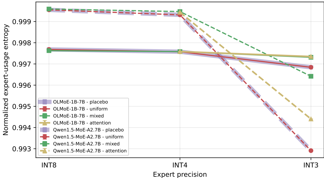
Normalized expert-usage entropy
