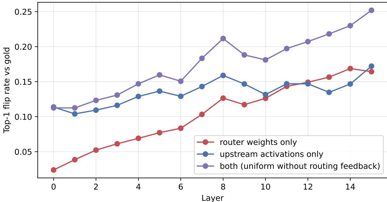
olmoe: mechanism split by layer at INT8
