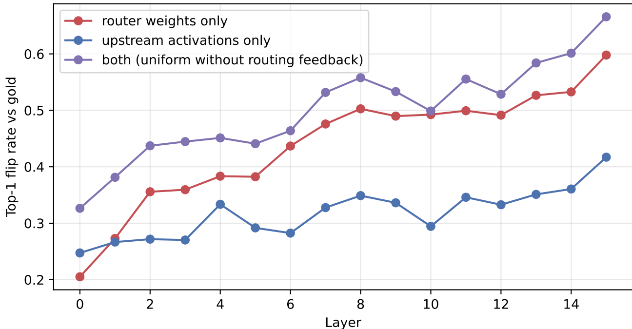
olmo: mechanism split by layer at INT3
