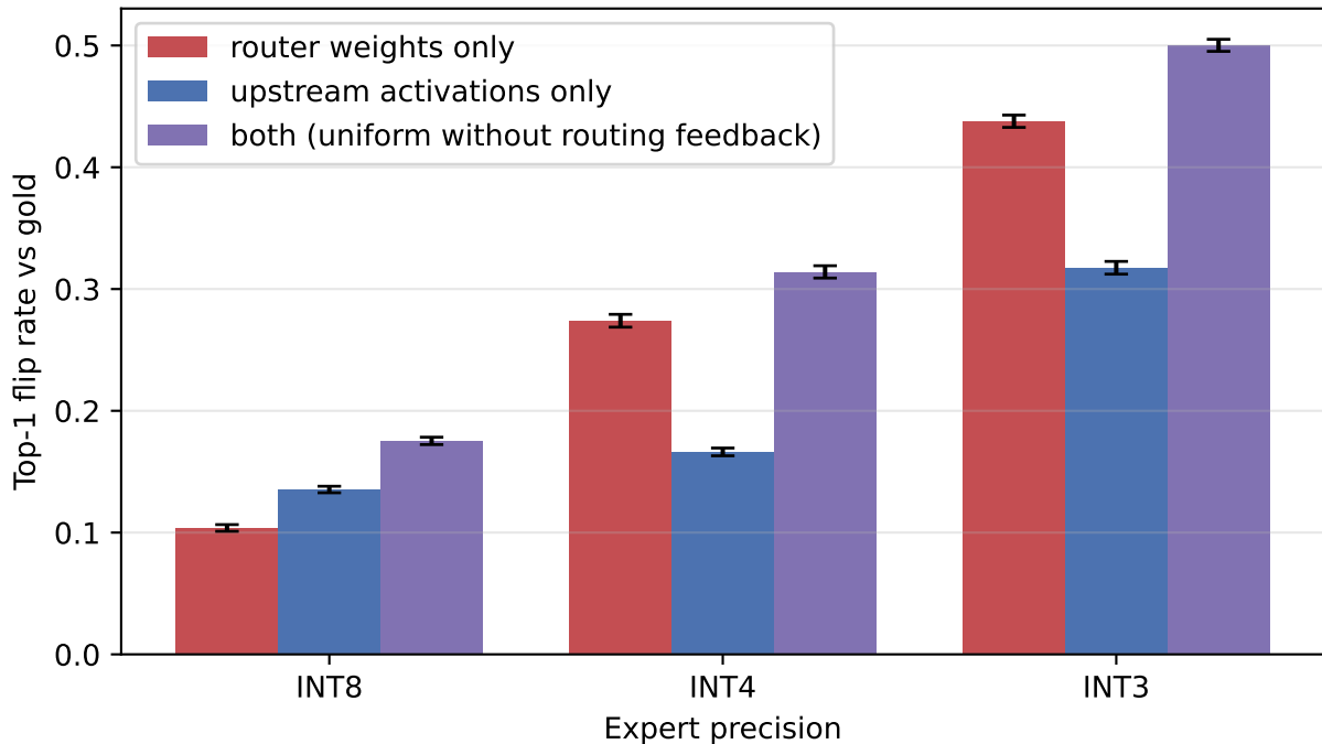
olmoe: where routing drift comes from
