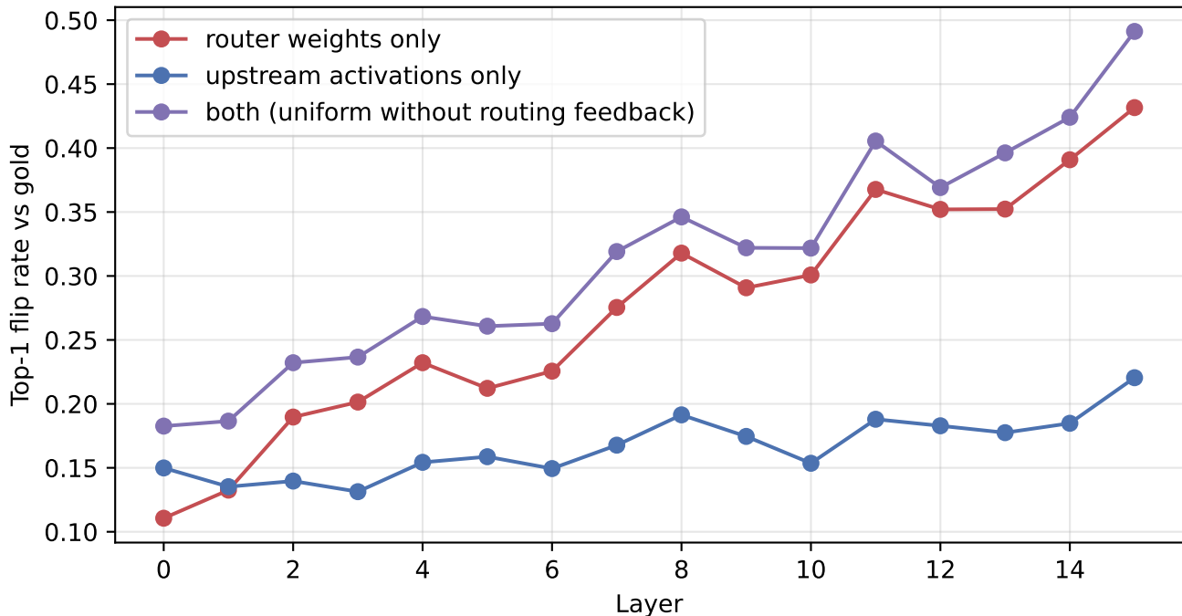
olmoe: mechanism split by layer at INT4
