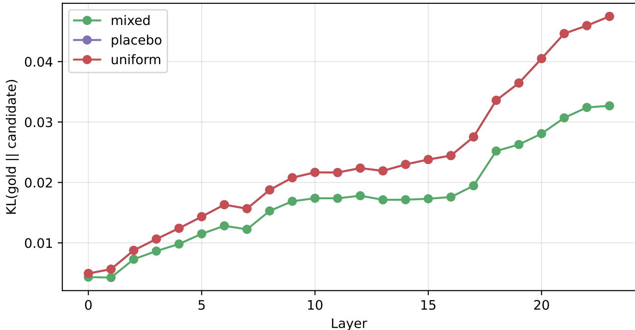
Layer-wise routing drift at INT8
