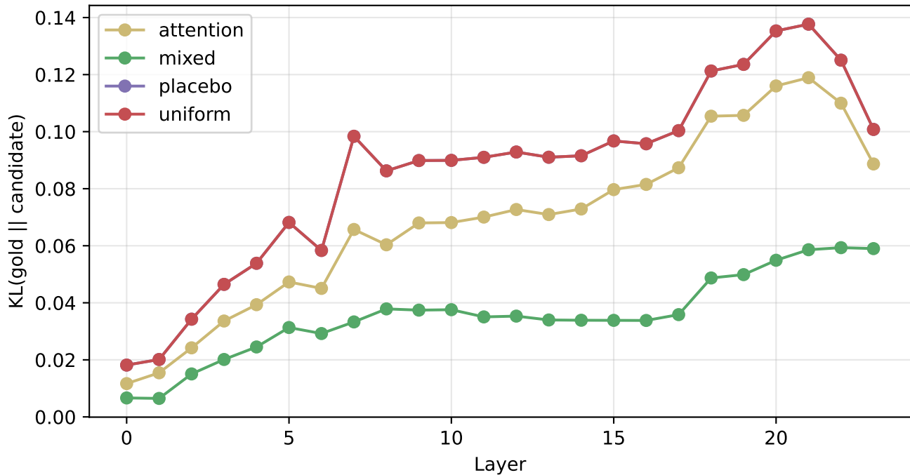
Layer-wise routing drift at INT4
