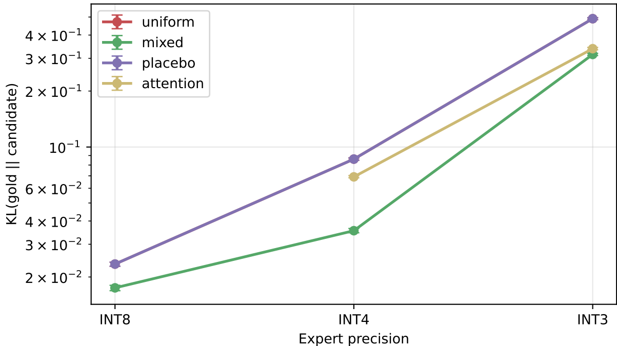
Routing drift vs expert precision
