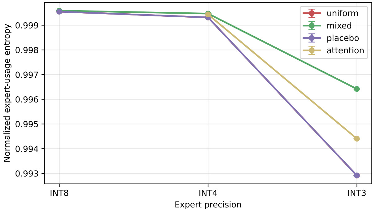
Expert collapse check
