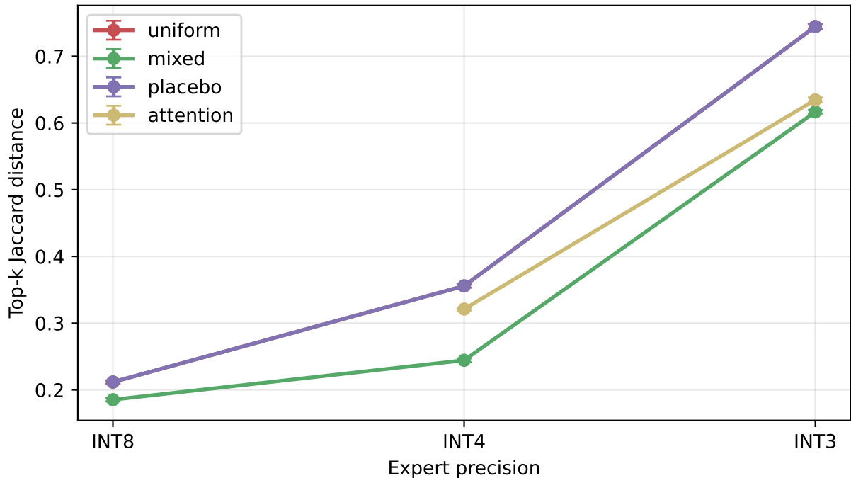
Expert-set disagreement vs precision
