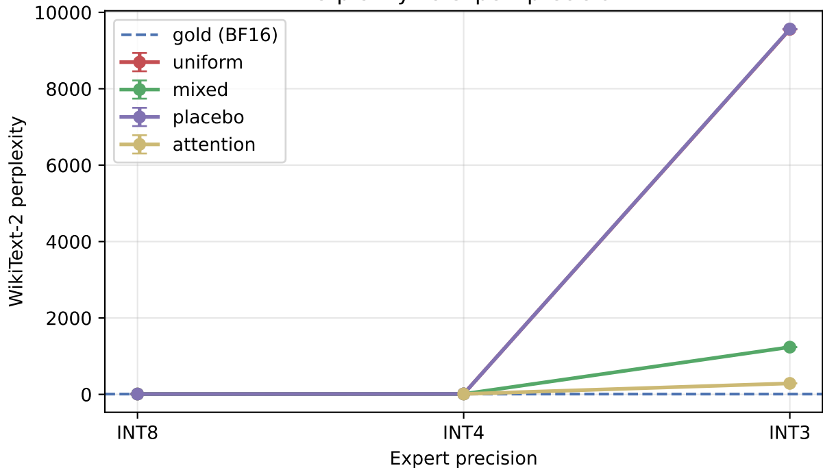
Perplexity vs expert precision
