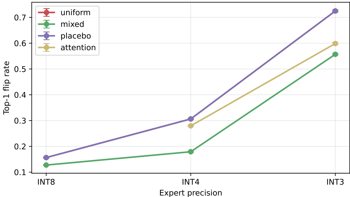
Top-1 expert changes vs expert precision
