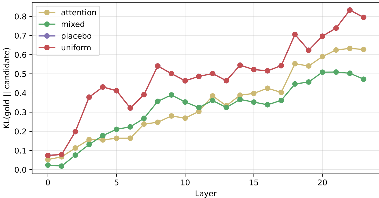
Layer-wise routing drift at INT3
