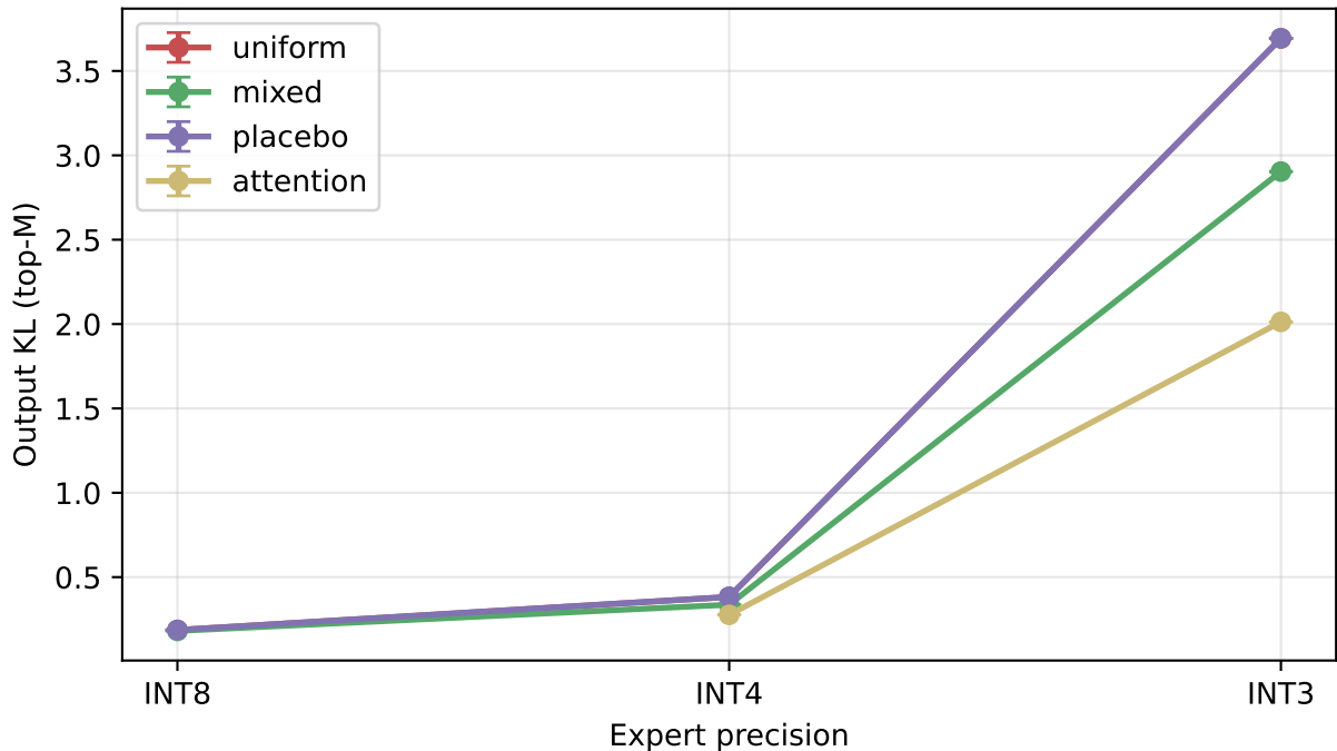
Output distribution drift vs precision
