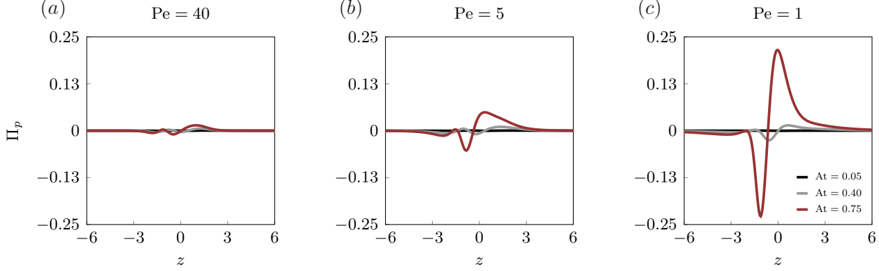
Figure 8: Pressure production \Pi_p(z) at k = 0.1 in the IDL formulation, showing when pressure work becomes dynamically important. (a) \text{Pe}_\delta = 40 . (b) \text{Pe}_\delta = 5 . (c) \text{Pe}_\delta = 1 .
