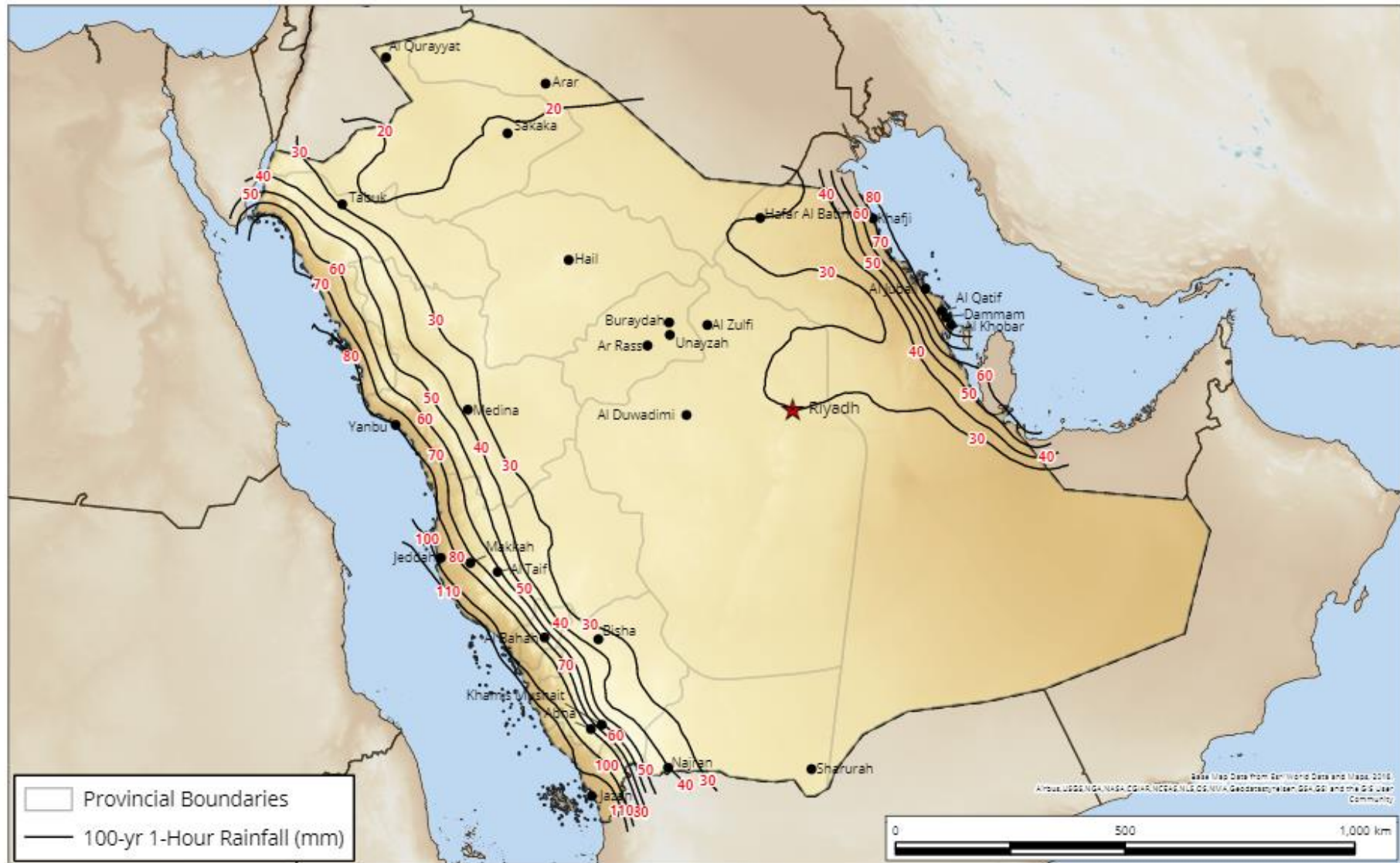
FIGURE 1106.1 100-YEAR, 1-HOUR RAINFALL (mm) OF SAUDI ARABIA
