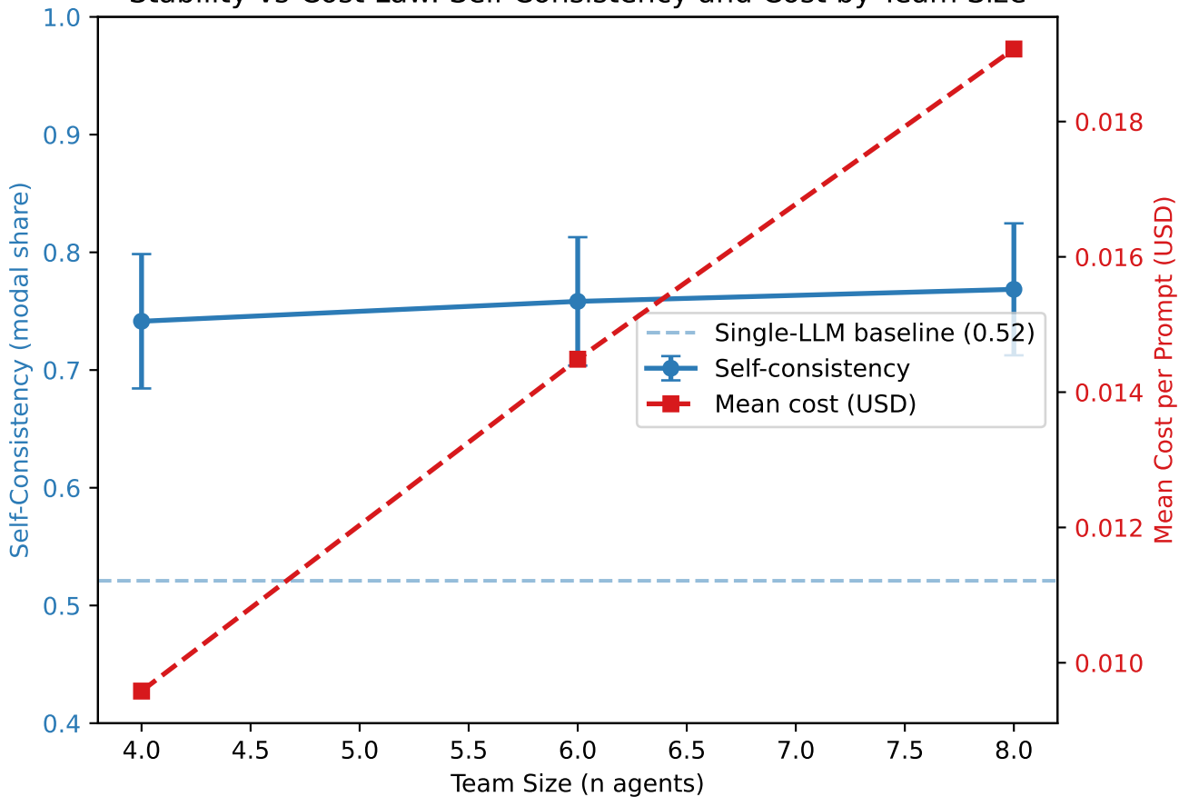
Stability-vs-Cost Law: Self-Consistency and Cost by Team Size
