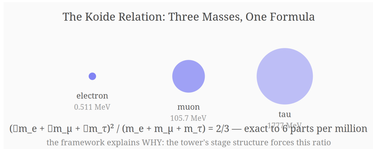
Figure 21: The Koide relation: three masses, one formula
