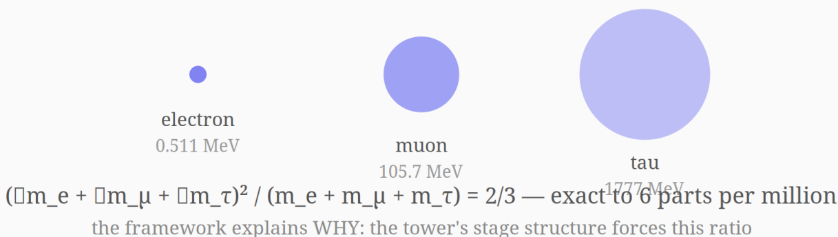
Figure 24: The Koide relation: three masses, one formula
