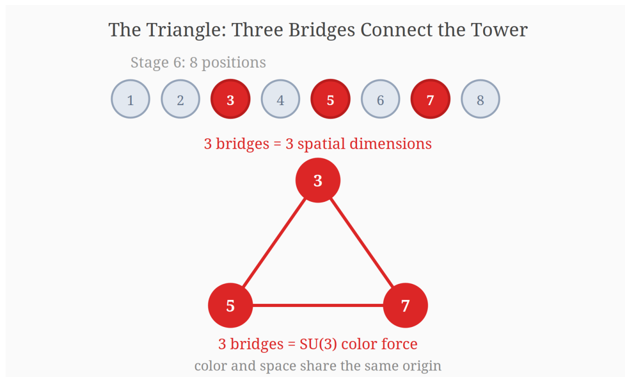
Figure 13: The three bridges form a triangle — the origin of both space and color
