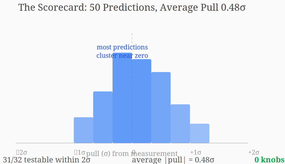
Figure 34: The scorecard: 50 predictions clustering near zero pull
