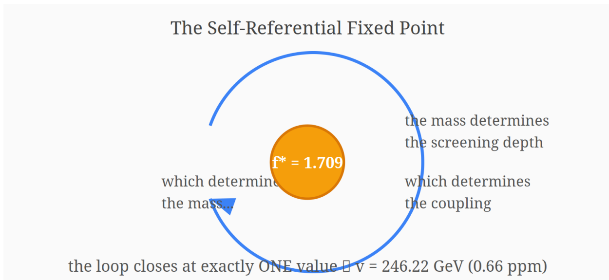
Figure 35: The self-referential fixed point: the mass determines its own screening
