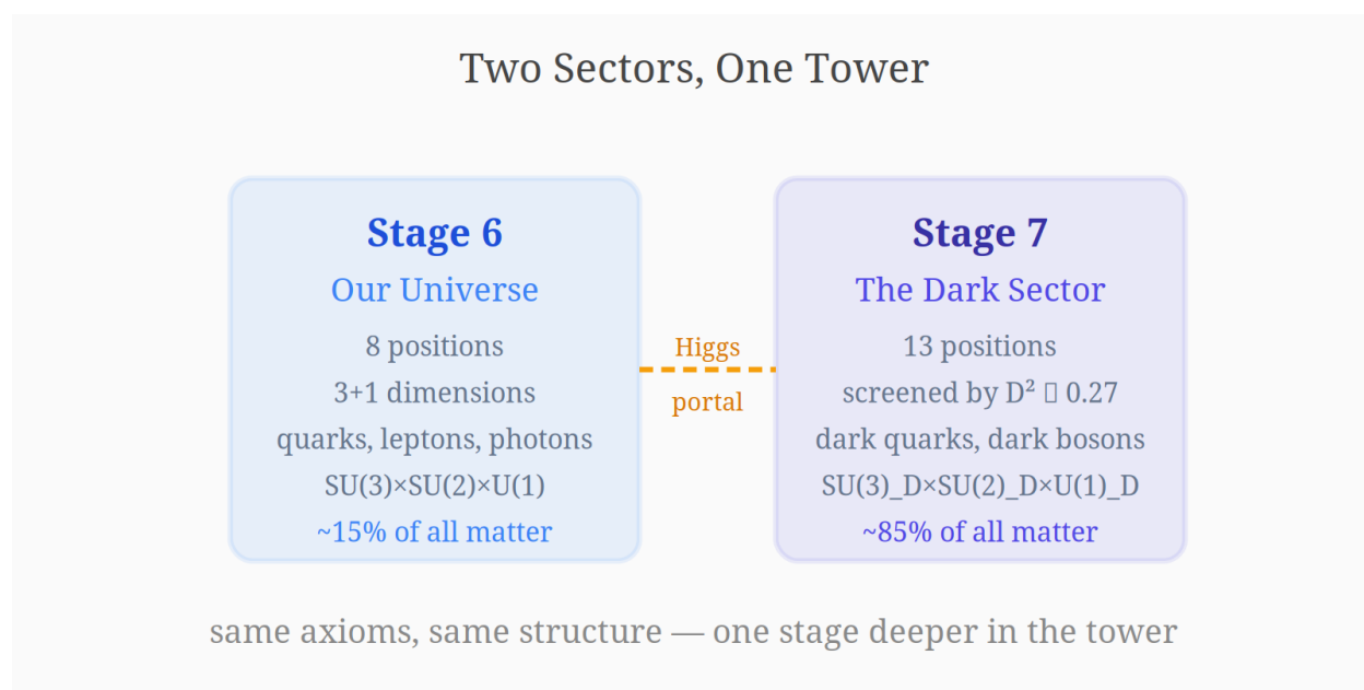
Figure 26: Two sectors, one tower: visible at stage 6, dark at stage 7
