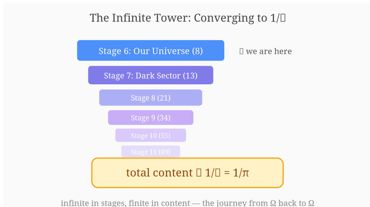
Figure 32: The infinite tower converging to 1/\pi
