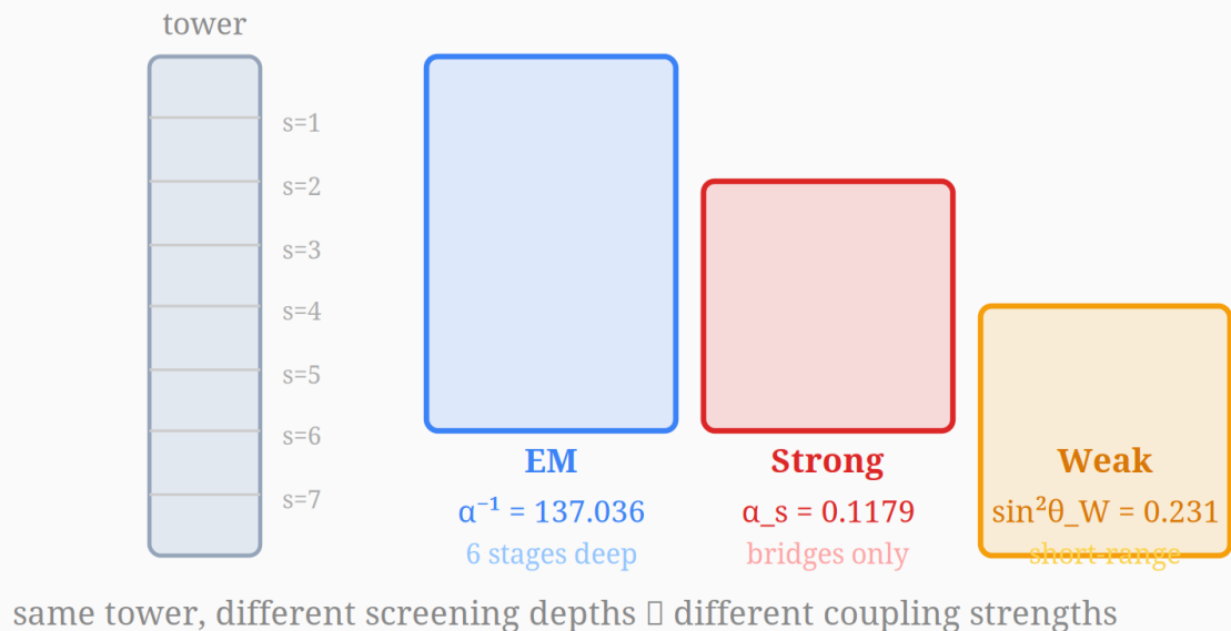
Figure 19: The three forces: one tower, three screening depths
