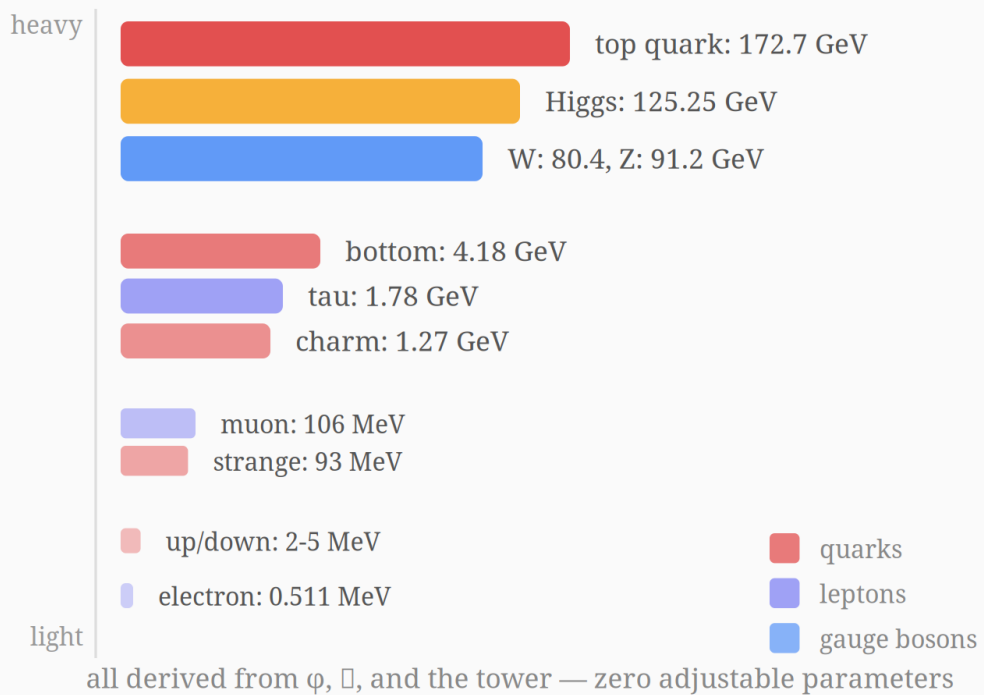
Figure 20: The mass ladder: every rung from the same ratio
