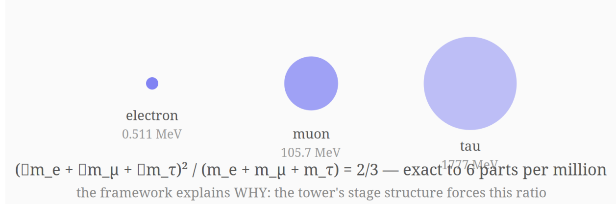
Figure 21: The Koide relation: three masses, one formula
