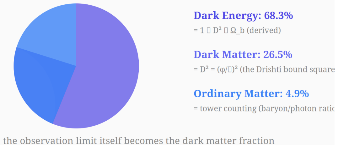
Figure 26: The energy budget: dark energy, dark matter, ordinary matter
