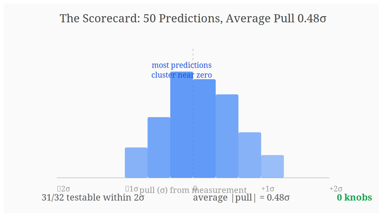
Figure 34: The scorecard: 50 predictions clustering near zero pull
