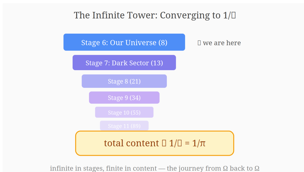
Figure 32: The infinite tower converging to 1/\pi
