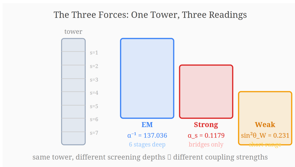
Figure 22: The three forces: one tower, three screening depths
