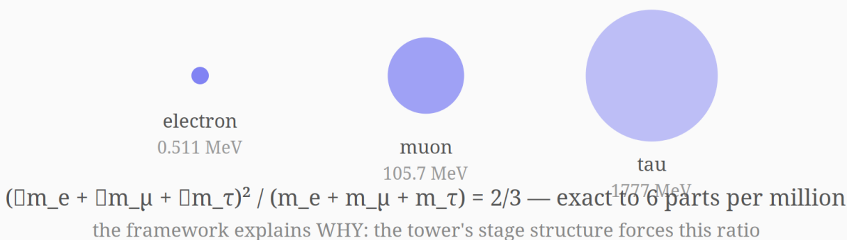
Figure 24: The Koide relation: three masses, one formula
